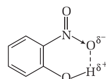
Intramolecular H-bonding in o -nitrophenol
